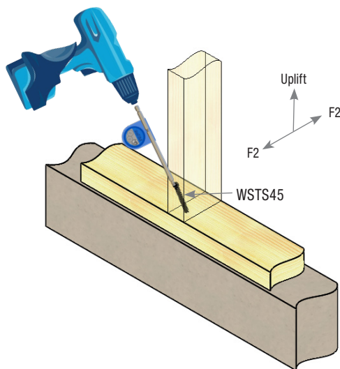
Typical WSTS45 stud-to-single bottom plate installation
