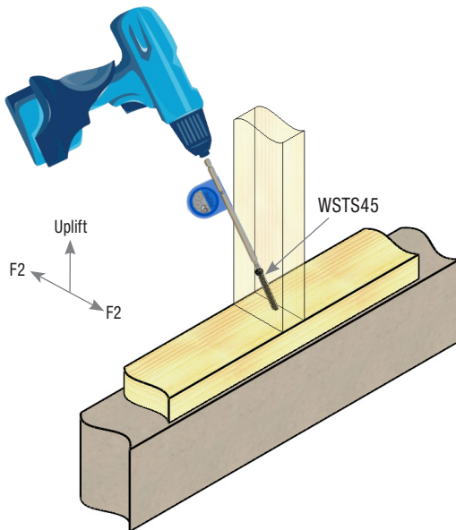
Typical WSTS45 stud-to-single bottom plate installation
