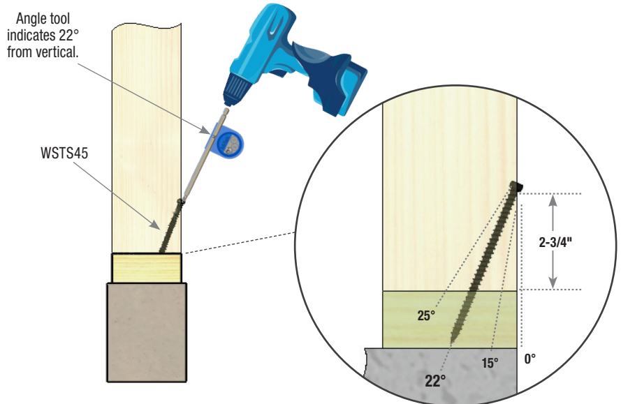
Narrow Face Installation
