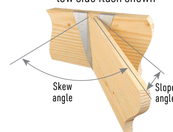
Figure 6 Joist Flush Options
