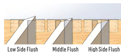
Figure 6 Joist Flush Options
