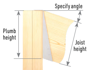
Figure 1 Sloped seat, down shown
