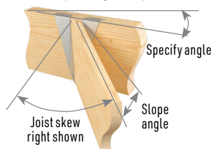
Figure 4 Skewed right, sloped down, top flange sloped
