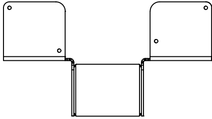
BPH3530 - TOP VIEW
