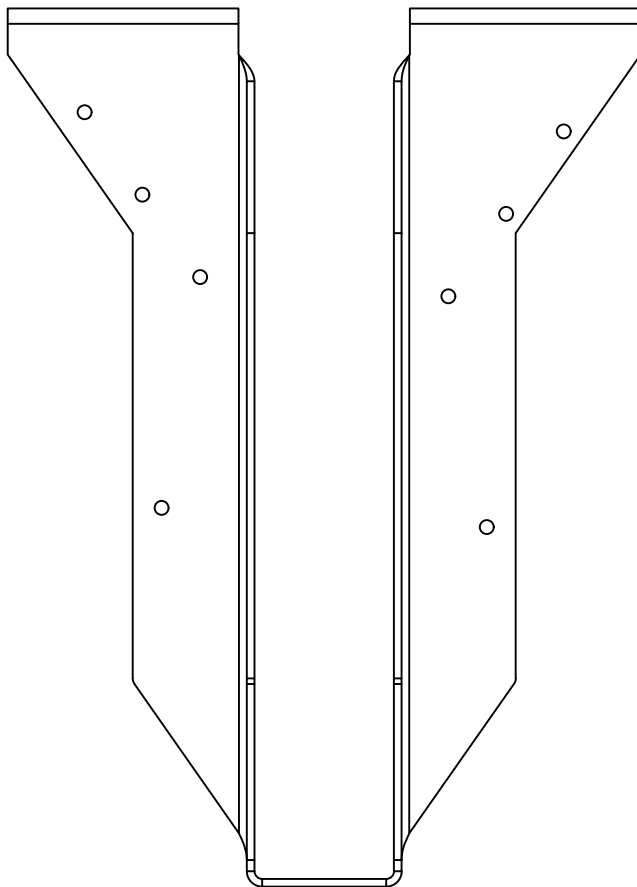
BPHA17112 - FRONT VIEW
