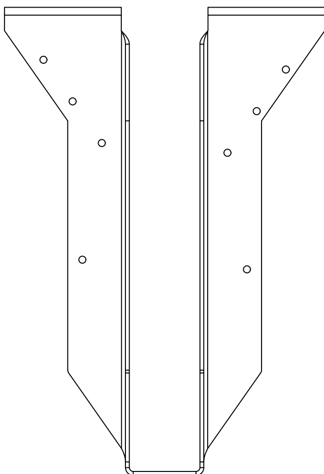
BPHA17118 - FRONT VIEW
