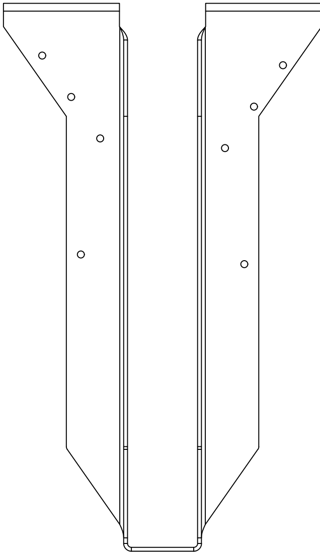
BPHA1714 - FRONT VIEW
