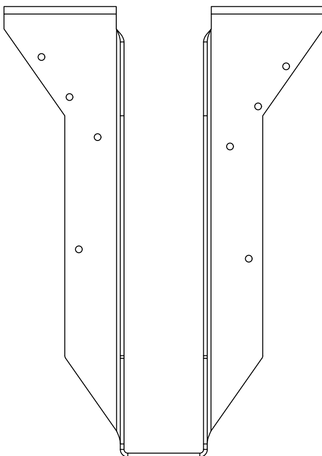
BPHA20118 - FRONT VIEW
