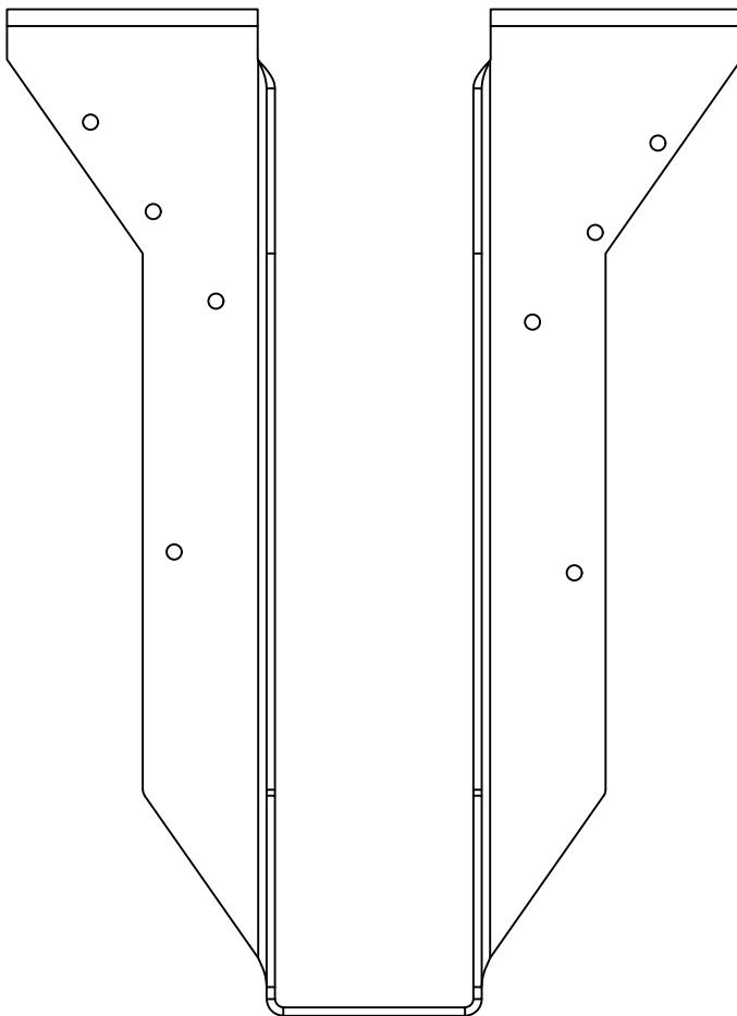
BPHA23118 - FRONT VIEW
