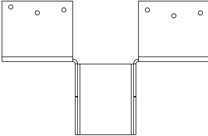
BPHA23118 - TOP VIEW
