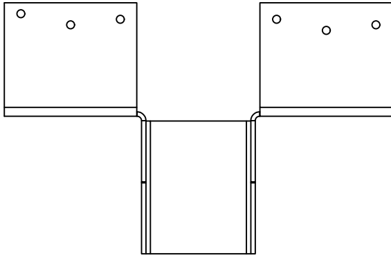
BPHA2316 - TOP VIEW
