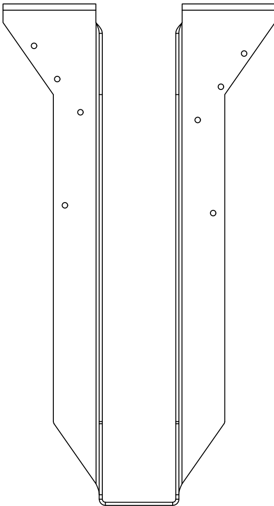
BPHA2316 - FRONT VIEW
