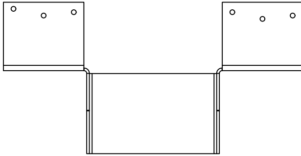
BPHA2320-2 - TOP VIEW
