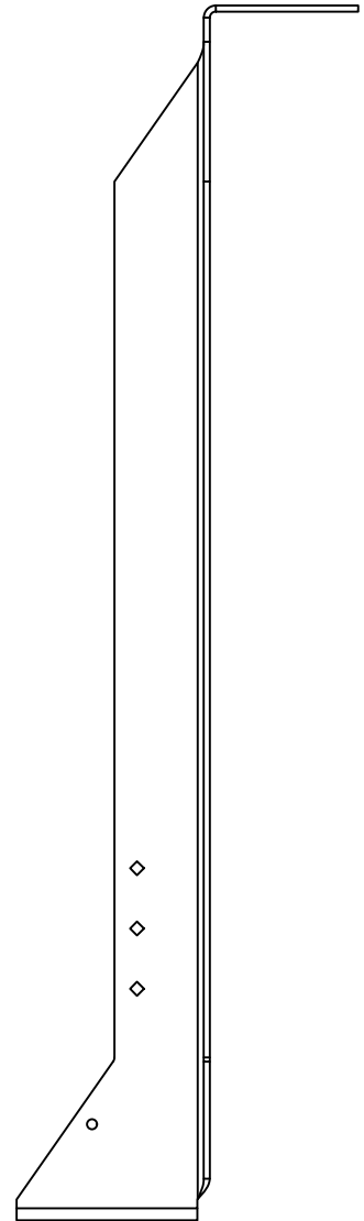
BPHA2320-2 - SIDE VIEW
