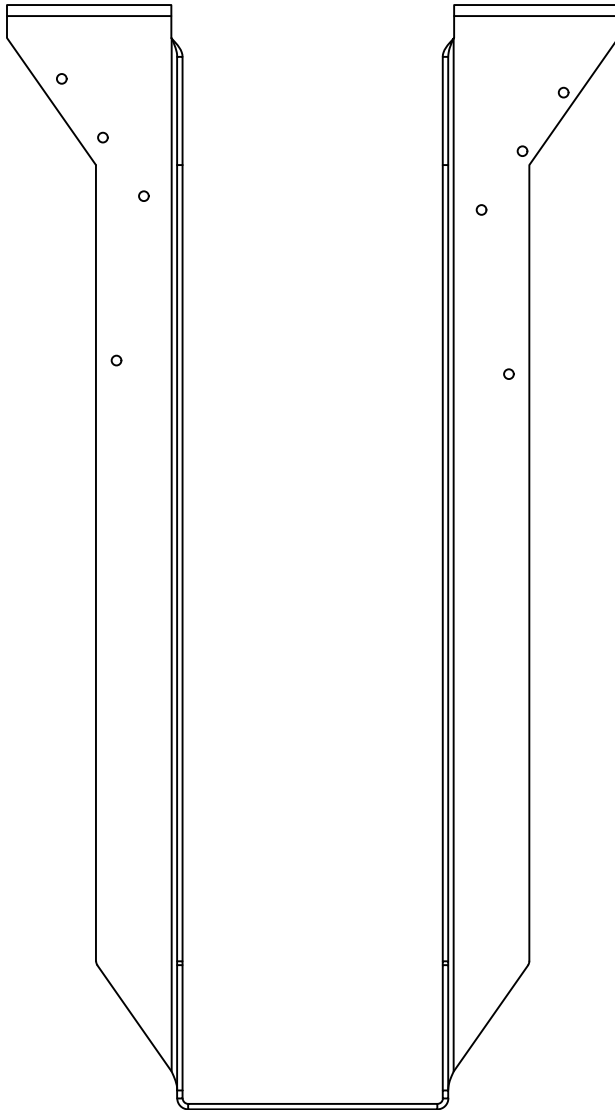
BPHA2320-2 - FRONT VIEW
