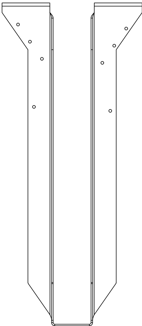
BPHA2320 - FRONT VIEW
