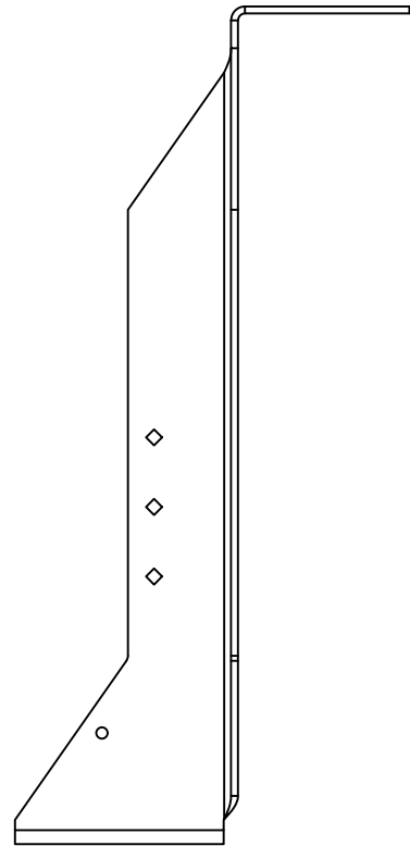
BPHA25118 - SIDE VIEW
