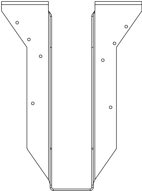
BPHA25118 - FRONT VIEW
