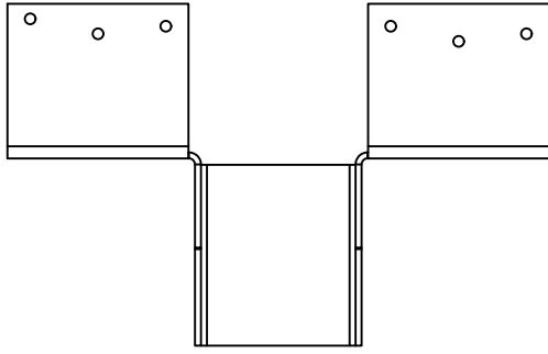
BPHA2522 - TOP VIEW
