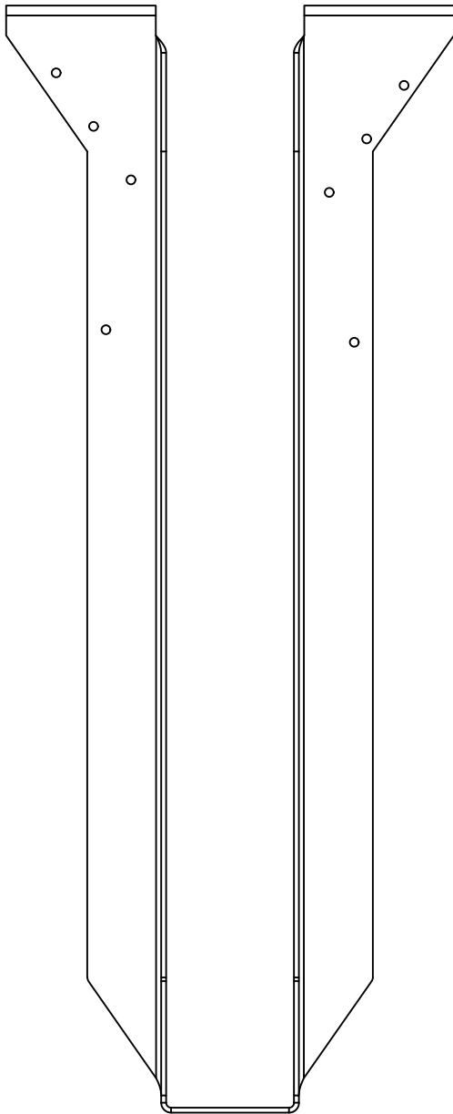
BPHA2522 - FRONT VIEW
