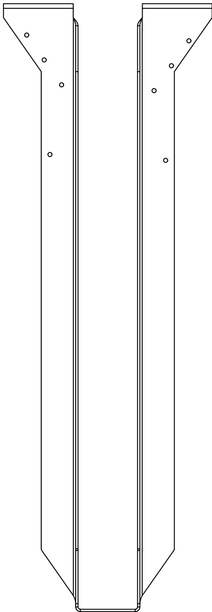
BPHA2526 - FRONT VIEW
