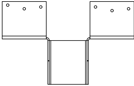
BPHA2526 - TOP VIEW
