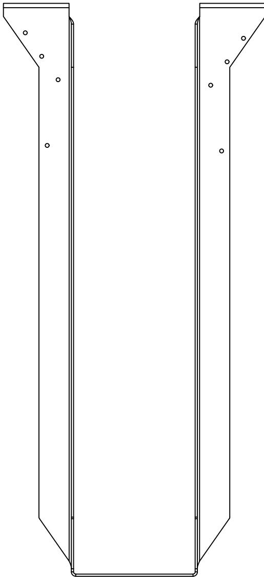
BPHA5526 - FRONT VIEW
