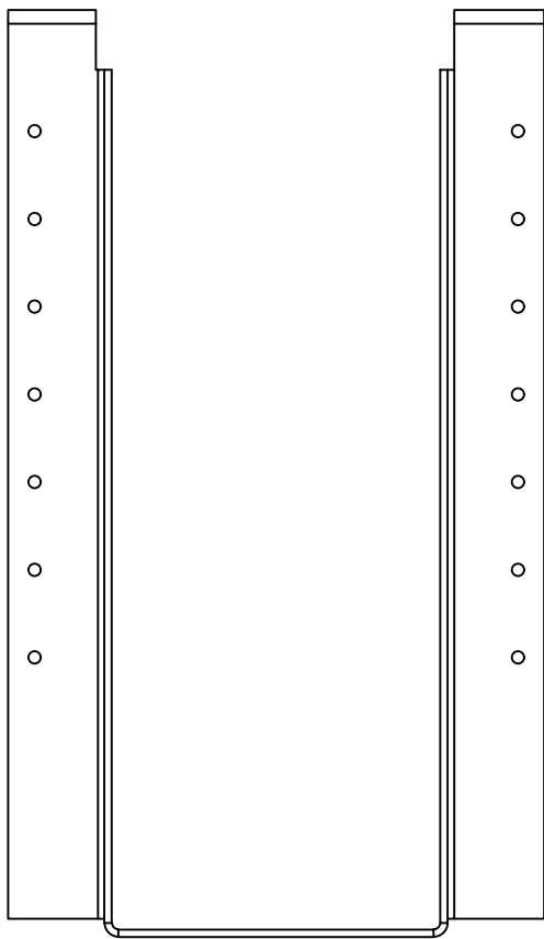
HDO214-3 - FRONT VIEW
