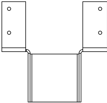
HDO310 - TOP VIEW
