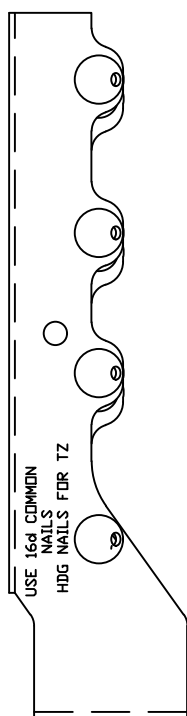
HUS210-2IF - SIDE VIEW
