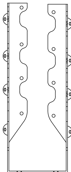
HUS210-2IF - FRONT VIEW
