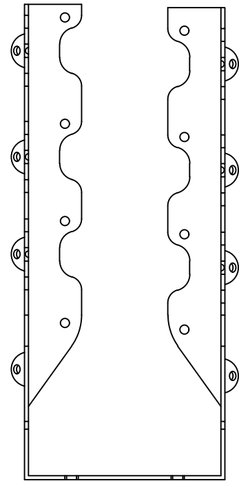
HUS410IF - FRONT VIEW
