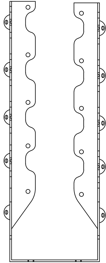
HUS412IF - FRONT VIEW
