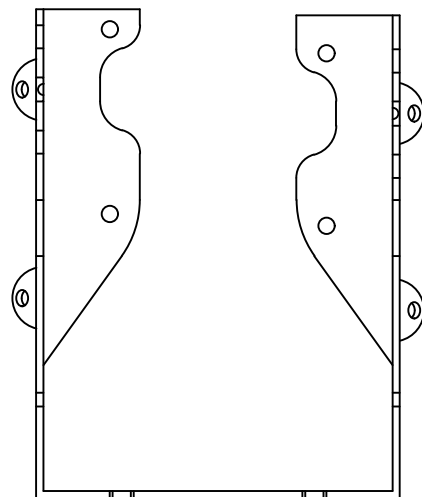
HUS46IF - FRONT VIEW
