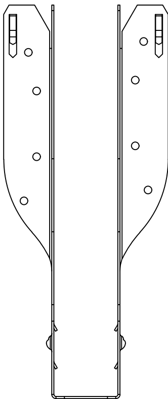
IHFL15925 - FRONT VIEW
