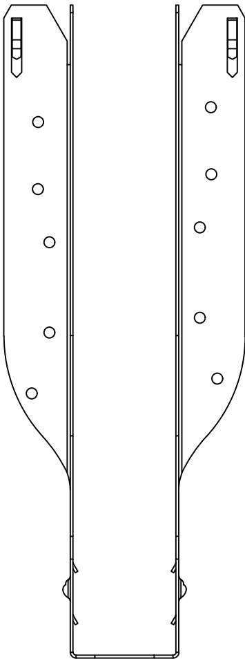
IHFL17112 - FRONT VIEW
