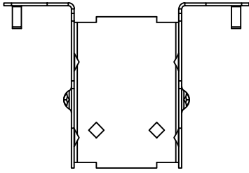
IHFL17112 - TOP VIEW
