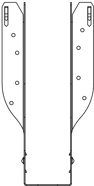
IHFL23925 - FRONT VIEW
