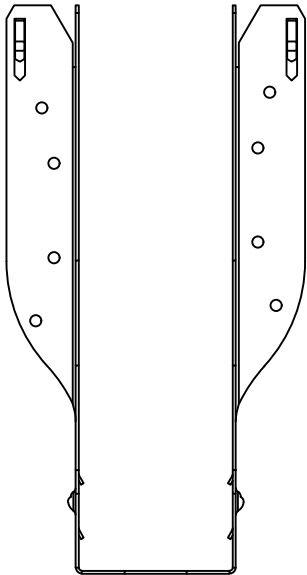
IHFL25925 - FRONT VIEW
