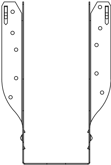
IHFL35925 - FRONT VIEW
