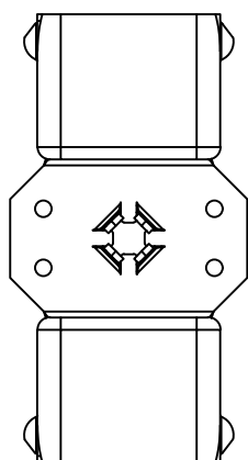
JDS24 - TOP VIEW
