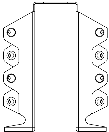
JDS26-175 - SIDE VIEW
