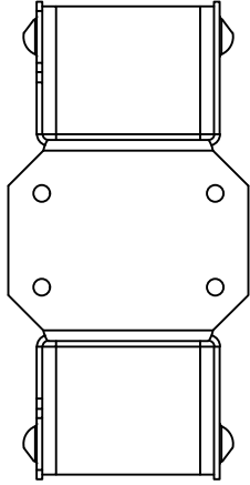
JDS26-175 - TOP VIEW
