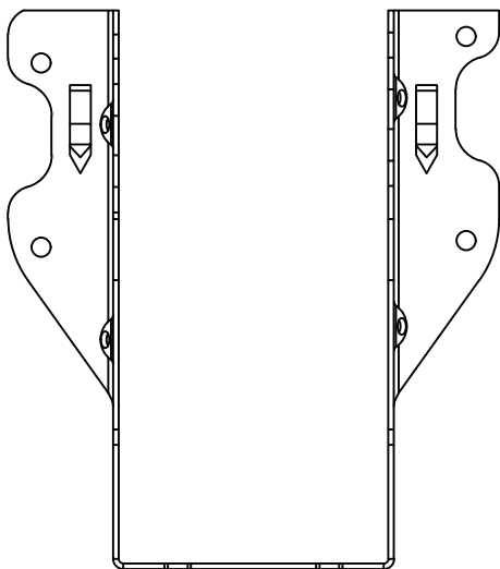
JUS36 - FRONT VIEW
