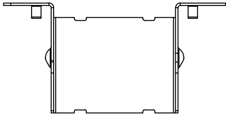
JUS36 - TOP VIEW
