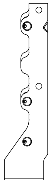
JUS410 - SIDE VIEW
