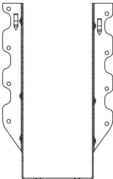
JUS410 - FRONT VIEW
