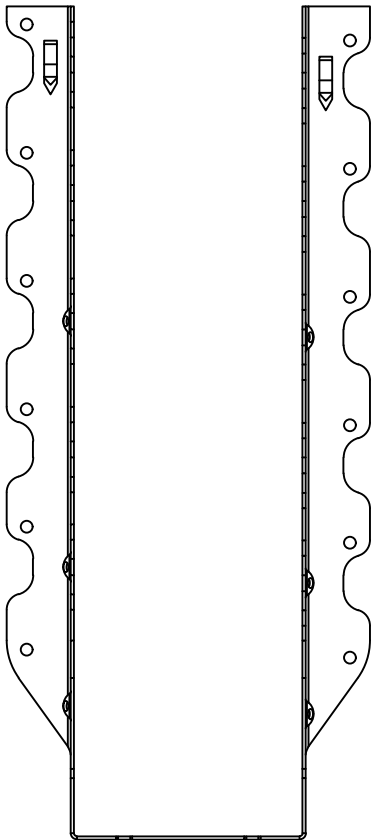
JUS414 - FRONT VIEW
