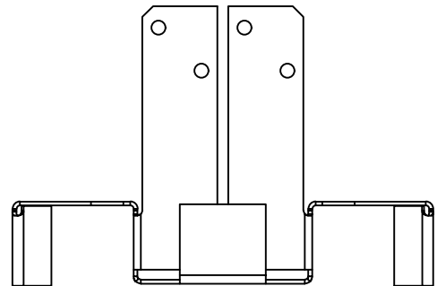
PAF66 - SIDE VIEW
