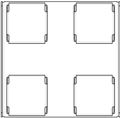
PAU1010R - TOP VIEW
