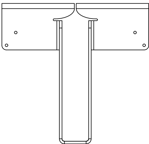
PHXU17925 - FRONT VIEW
