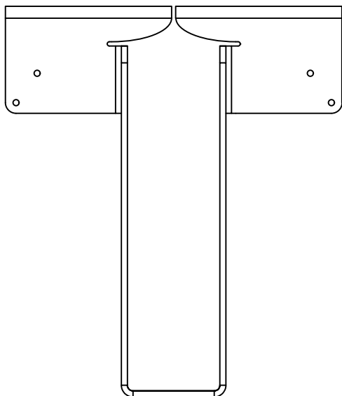
PHXU27112 - FRONT VIEW
