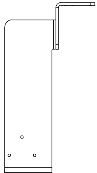
PHXU71112 - SIDE VIEW
