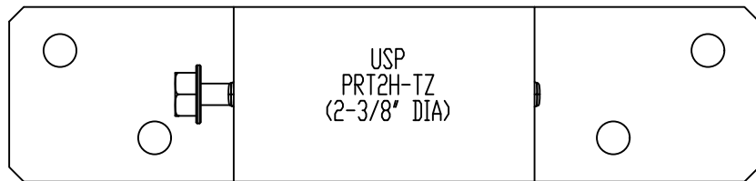
PRT2H-TZ - FRONT VIEW
