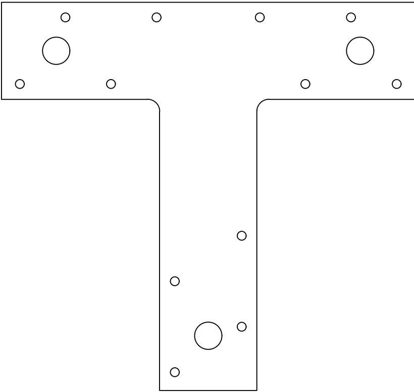
T8 - FRONT VIEW
