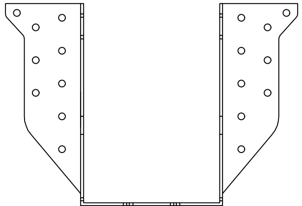
THD46 - FRONT VIEW
