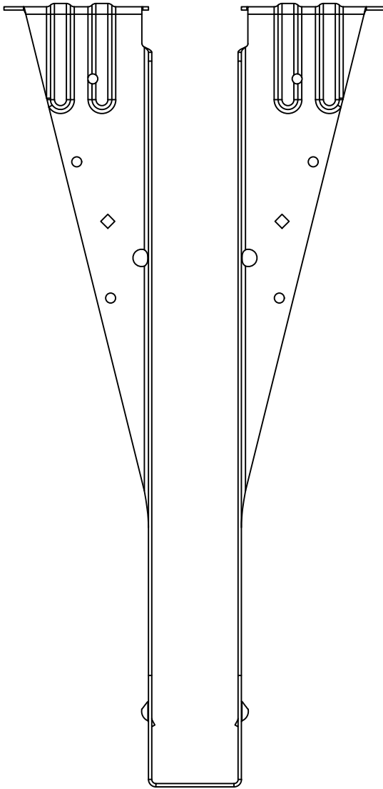
THO15140 - FRONT VIEW
