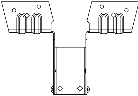
THO15140 - TOP VIEW
