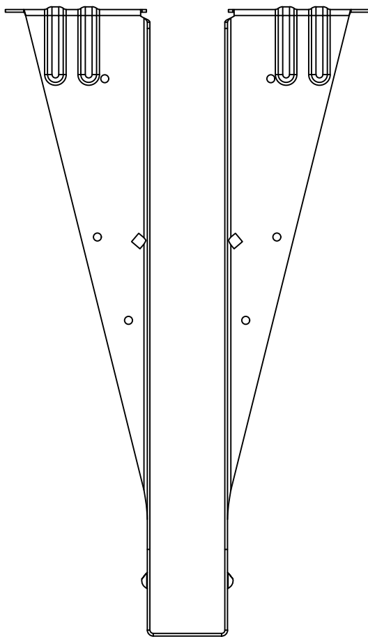
THO16140 - FRONT VIEW
