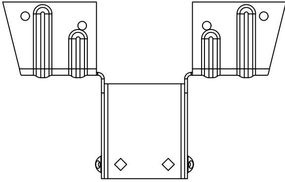
THO16950 - TOP VIEW
