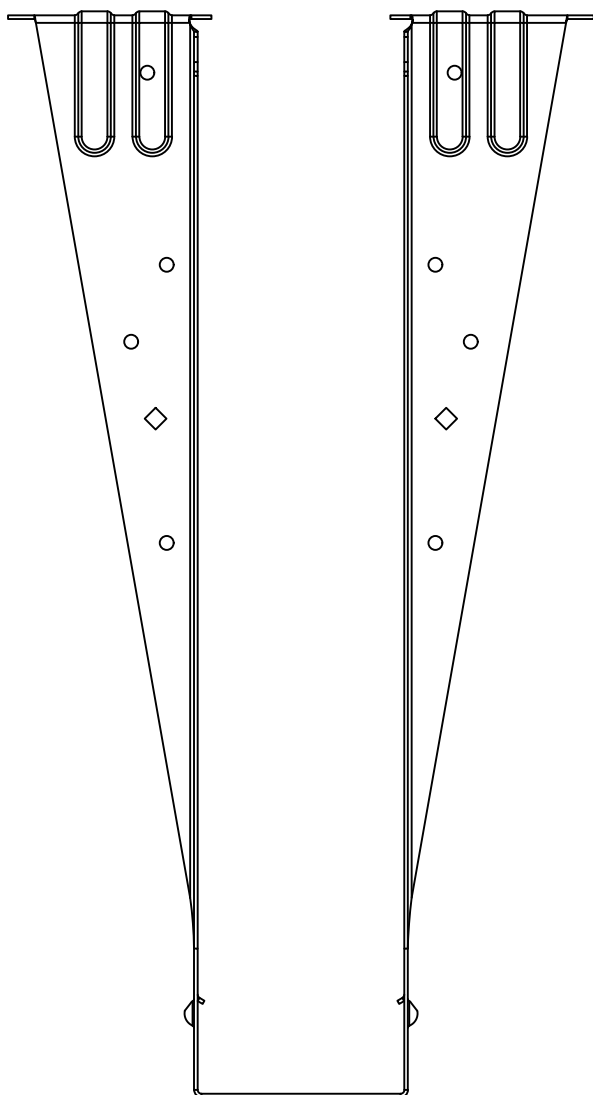
THO26140 - FRONT VIEW
