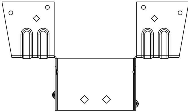
THO35130 - TOP VIEW
