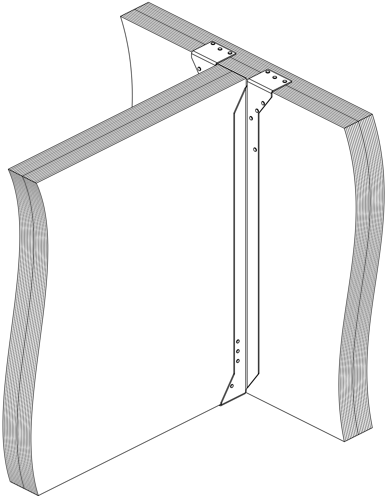
MITEK BPHA3532 (Maximum Nailing)
