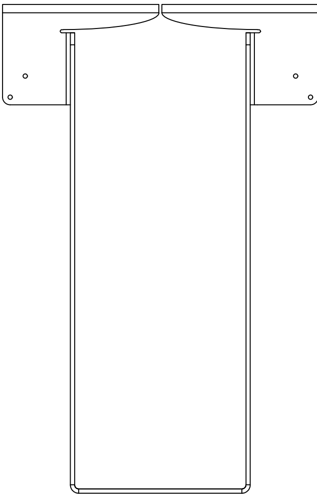
PHXU7120 - FRONT VIEW
