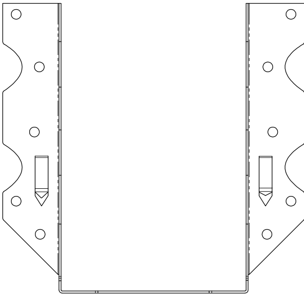
SUH46 - FRONT VIEW
