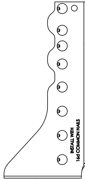
THDH610 - SIDE VIEW
