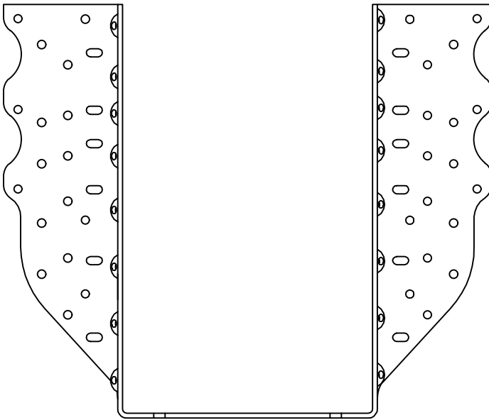
THDH610 - FRONT VIEW
