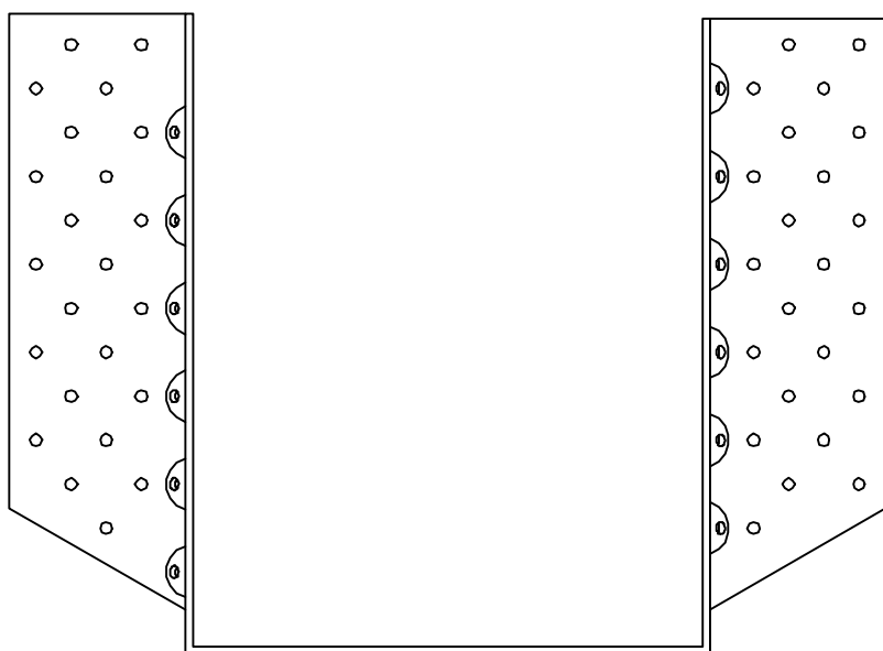
THDH7210 - FRONT VIEW
